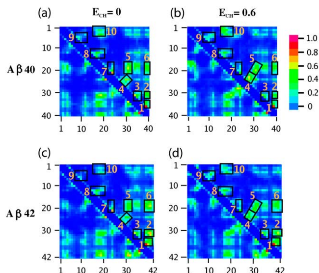
FIGURE 4 Intramolecular contact maps of folded A \beta 40 and A \beta 42 monomers at E_{CH} = 0 (left column) and E_{CH} = 0.6 (right column). The strength of the contact map is color-coded following the rainbow scheme: from blue (no contacts) to red (the largest number of contacts). Each contact map is an average of over 100 monomer conformations after 1,000,000 simulation steps.
