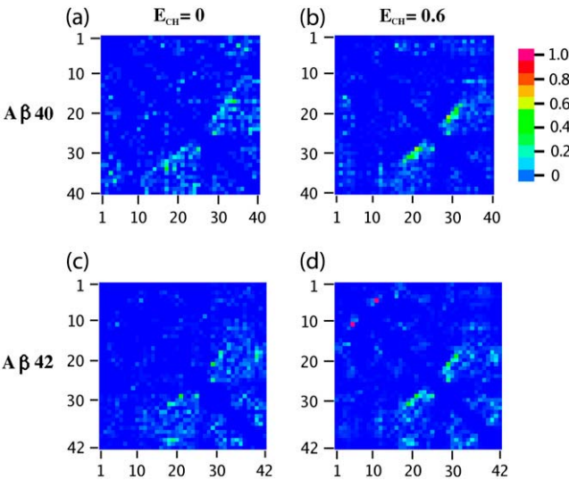
FIGURE 10 Intramolecular hydrogen bond maps of A \beta 40 and A \beta 42 pentamers and larger oligomers at E_{CH} = 0 and E_{CH} = 0.6 . Each map is an average of >50 conformations at 8, 8.5, 9, 9.5, and 10 million simulation steps.
