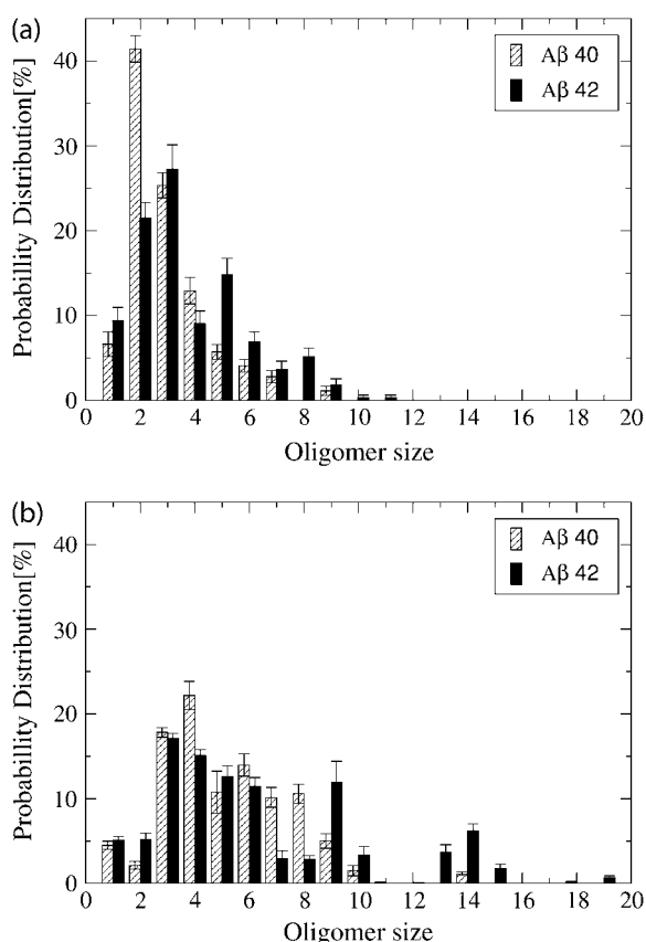
FIGURE 2 Oligomer size distributions of A \beta 40 and A \beta 42 at (a) E_{CH} = 0 and (b) E_{CH} = 0.6 . All size distributions are averages over the time frames at 8, 8.5, 9, 9.5, and 10 million simulation steps.
